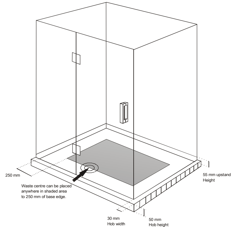
Indicative illustration of Freeform shower base & system.
