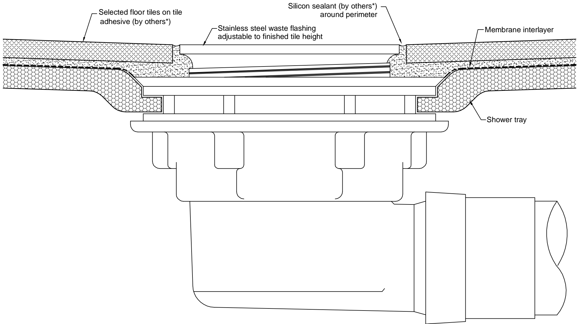
DETAIL 5 01 WASTE OUTLET (to fit Easyclean waste outlet)
