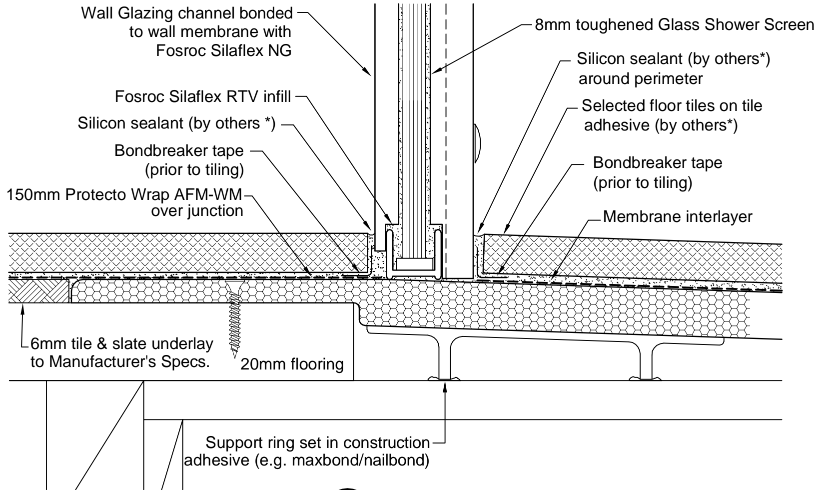
DETAIL 4 01 WALL / FLOOR INTERSECTION Level Tray
