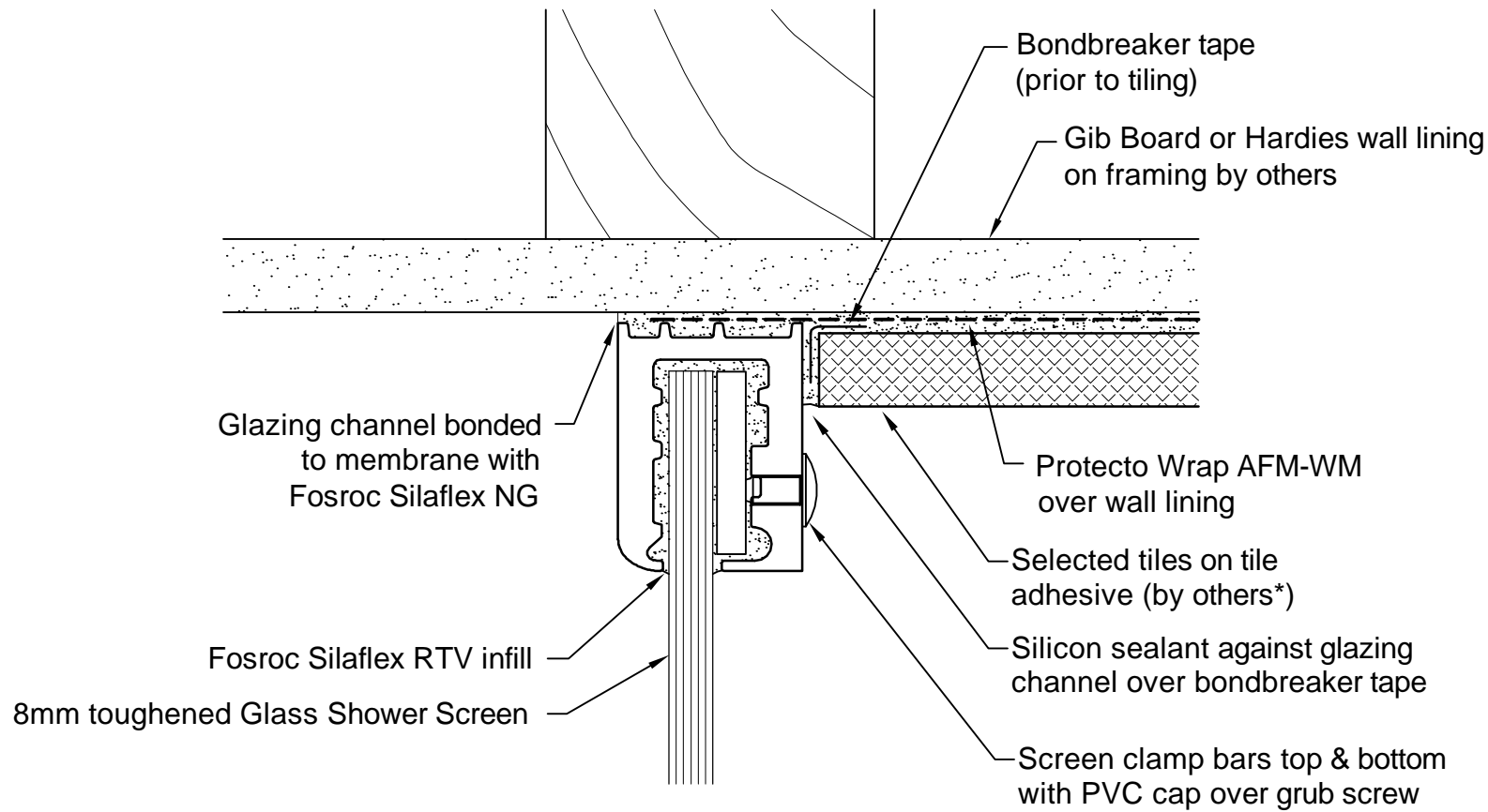
DETAIL 3 WALL to SHOWER SCREEN 01
