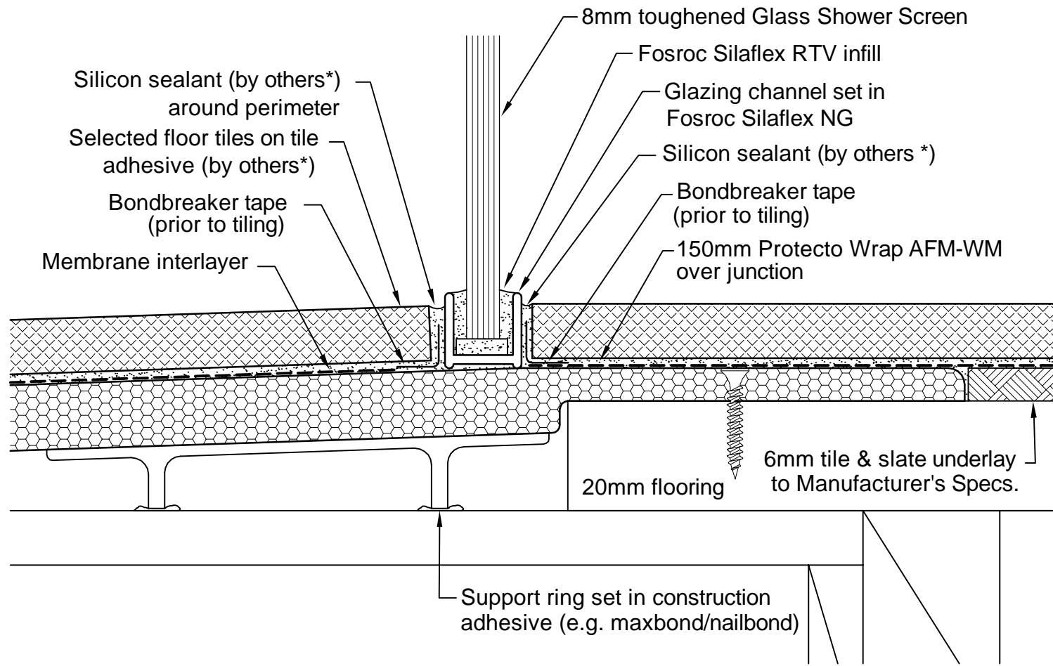
DETAIL 1 01 SHOWER SCREEN TO LEVEL TRAY
